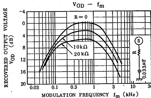
Graph 2 VOD - fm
