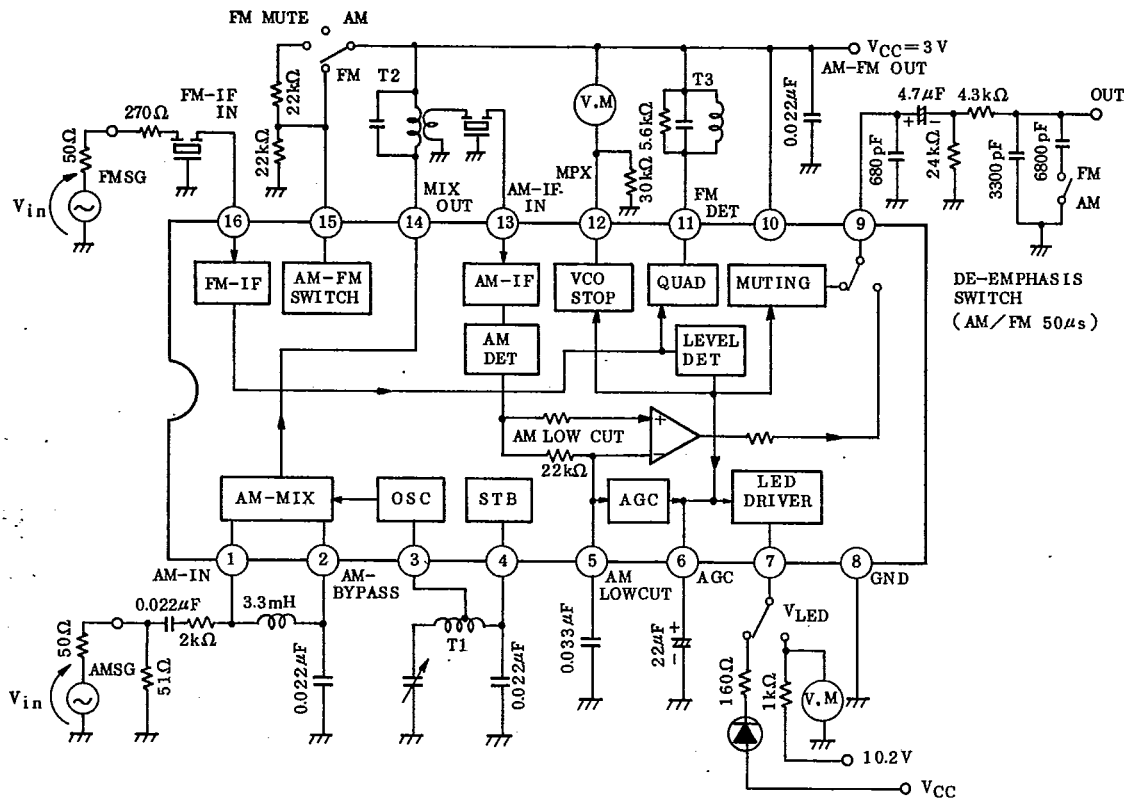
TEST CIRCUIT 1
